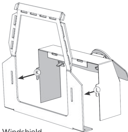
Part F: Windshield
